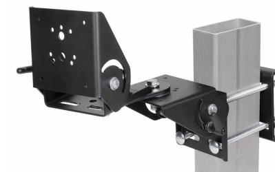
7160-0420 Dual Clam Shell with Arm and Small Backer Plate
