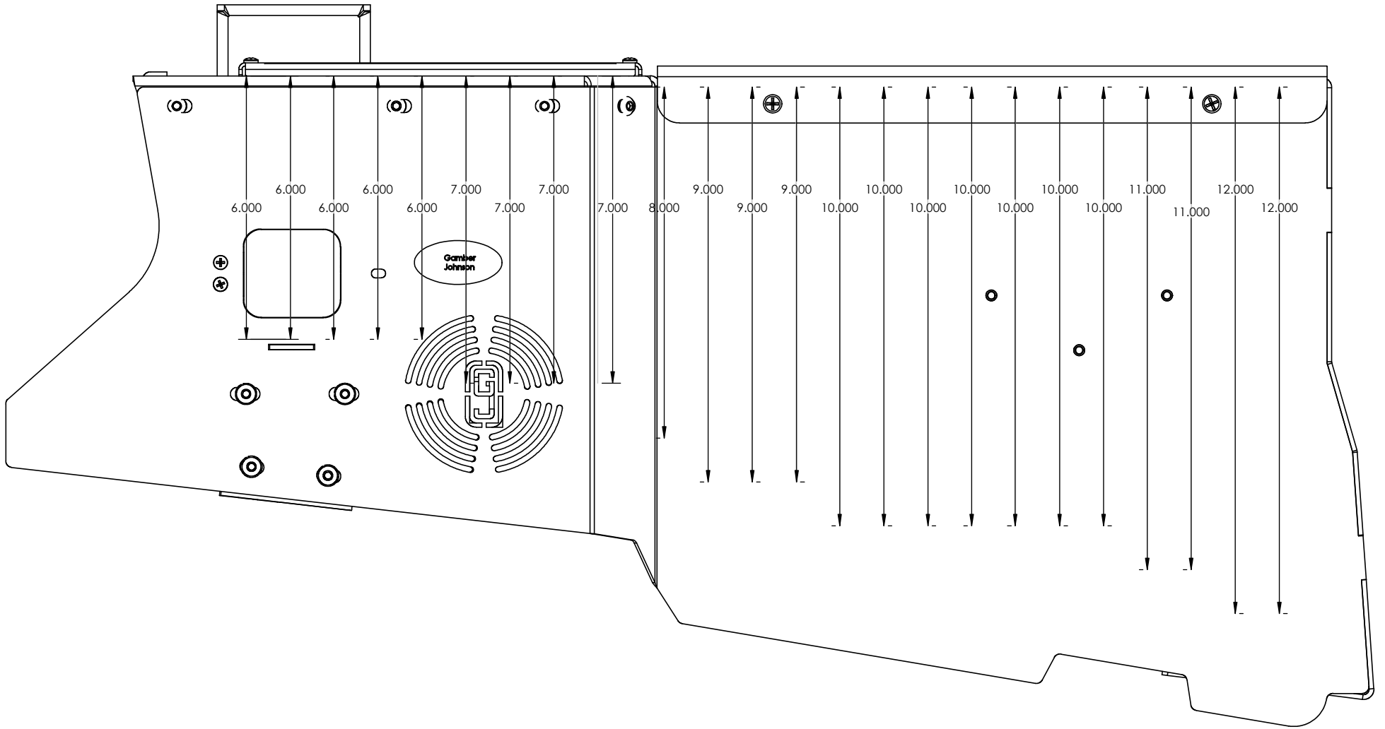
SIDE MOUNT DIMENSIONS
