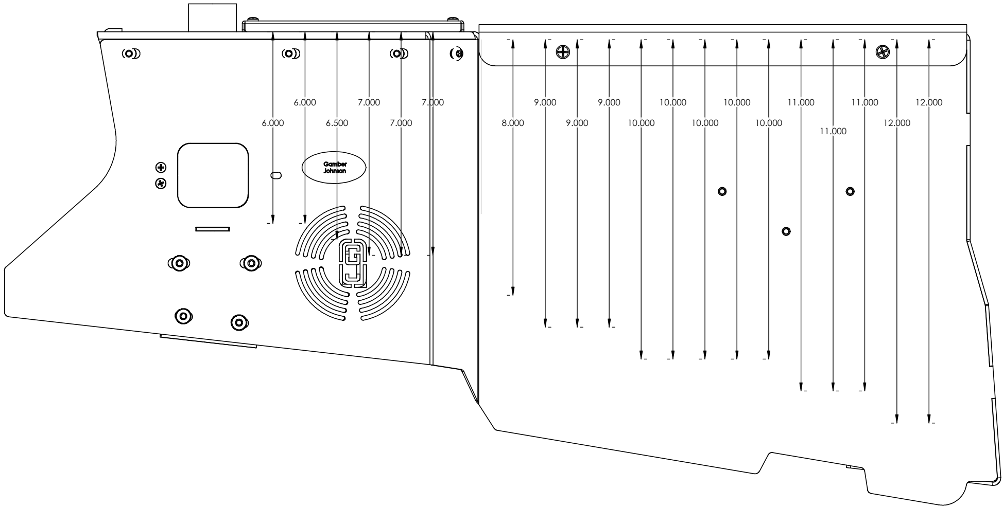
CENTER MOUNT DIMENSIONS
