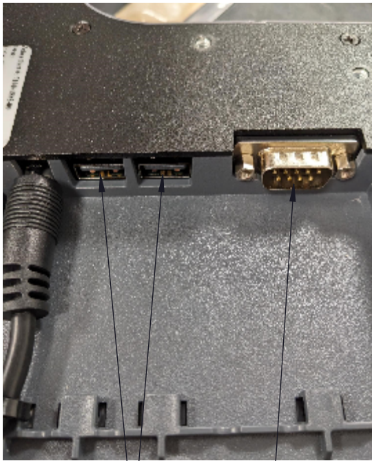
— RS232 SERIAL — USB 2.0 TYPE A
