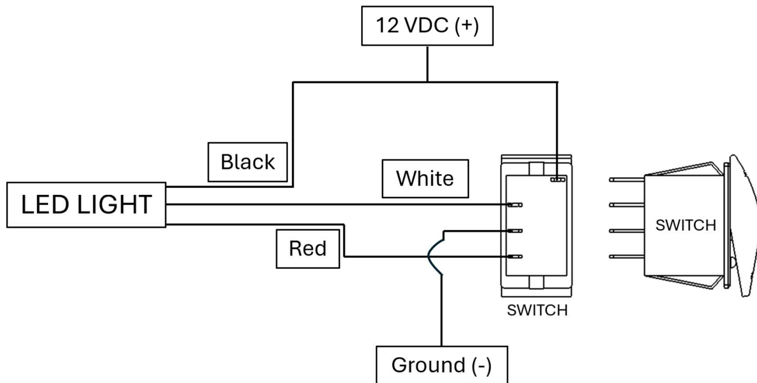
Console Box Light Wiring Diagram
